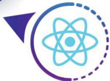
React Native
